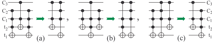
Figure 4: Toffoli templates.
